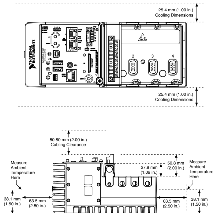
Figure 1. NI cDAQ-9132 Temperature, Cooling, and Cabling Dimensions
