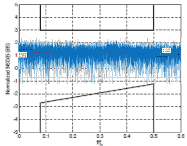
Figure 9: Noise Flatness
