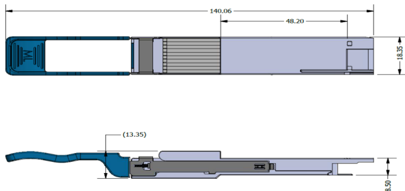
Figure 10: Mechanical Dimensions
