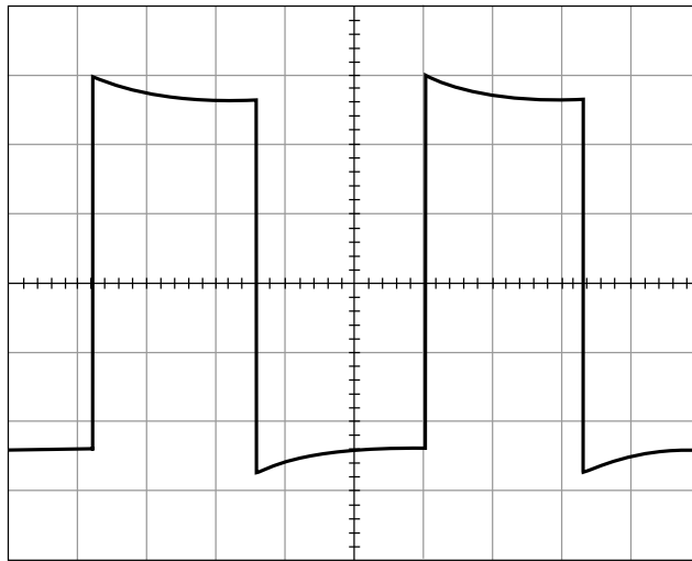
Figure 4. Overcompensated Square Wave Response
