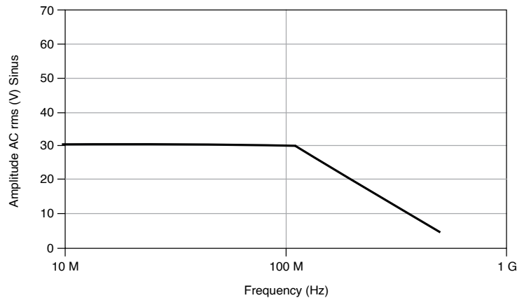
Figure 2. CP400X and CP500X Typical Voltage Derating
